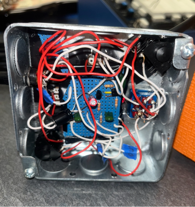
FIG. 5: An image of the final circuit in its enclosure.
